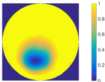
(c) EIDORS [1]
