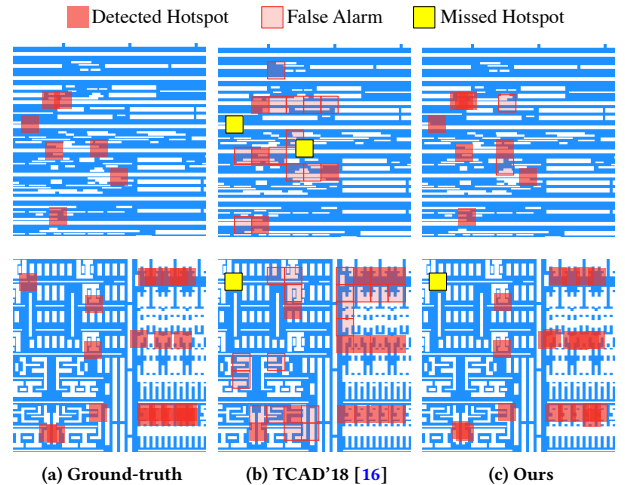
Figure 9: Visualization of different hotspot detection results.
