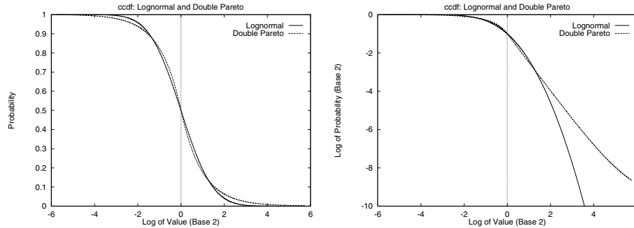
Figure 1. Shapes of lognormal and double Pareto distributions.
