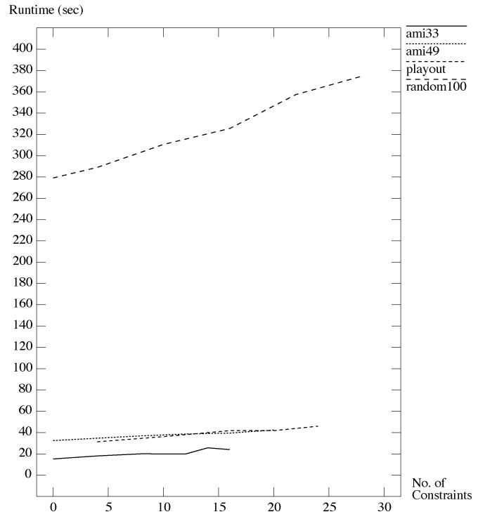
Fig. 18. Relationship between runtime and the number of placement constraints.
