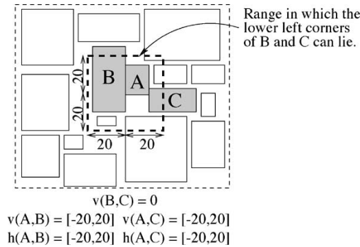
Fig. 10. Example of an arbitrarily set of mixed constraints.
