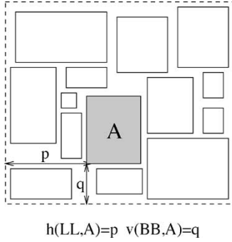
Fig. 6. Examples of preplace constraint.
