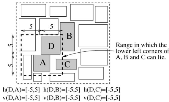
Fig. 9. Examples of clustering constraint.
