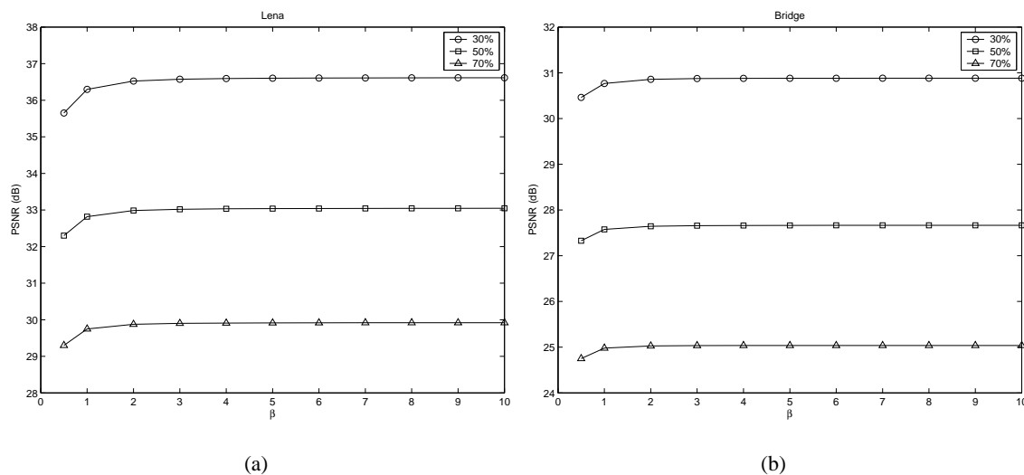
Fig. 6. PSNR of restored images by our Algorithm III for different \beta : (a) Lena image and (b) Bridge image.
