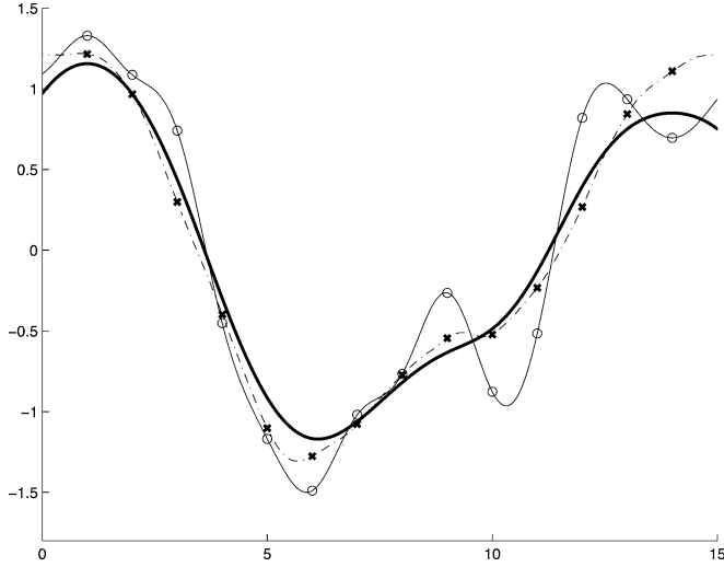
Fig. 2. Example of continuous-time signal estimation from discrete noisy data. The underlying third-order continuous-time process x(t) is displayed in dotted lines, and its noise-free samples are marked by crosses. The noisy input samples are shown as circles. The thin continuous curve is the corresponding interpolating L*L-spline. The optimal smoothing spline (thicker line) is comparatively much closer to the noise-free reference signal.
