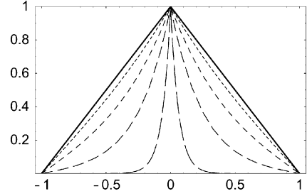
Fig. 1. Optimal interpolation kernels associated with the first-order differential operators L = D - \alpha I . The corresponding parameter values from top to bottom are \alpha = 0 (piecewise linear interpolator) and \alpha = \pm 1, \pm 2, \pm 4, \pm 16 . The magnitude of \alpha controls the degree of concavity of the curve and its peakedness at the origin, while the sign has no influence.
