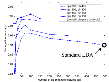
Figure 9. Accuracies using different number of discriminant features extracted from intrapersonal subspace.
