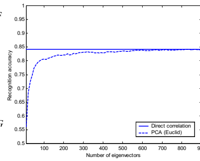
Figure 5. Recognition accuracy of the PCA method on the FERET database.
