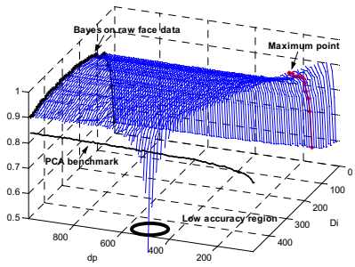
Figure 7. Accuracy curves for Bayesian analysis in PCA space.
