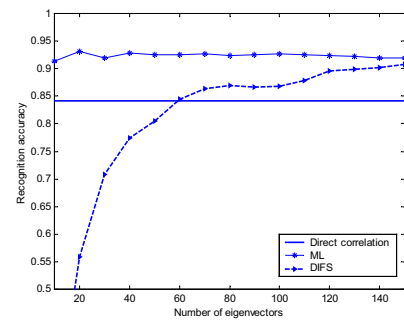
Figure 6. Recognition accuracy of the Bayesian algorithm on the FERET database.
