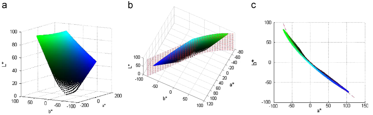
Fig. 3. (a) 256 \times 256 colors \{R_{Ar} = 0, G_{Ar} = 0, 1, \dots, 255, B_{Ar} = 0, 1, \dots, 255\} in the CIELAB color space. (b) The approximation surface modeled by Eq. (9) and indicated by the red dashed lines. (c) Top views of the original and the approximation surface.
