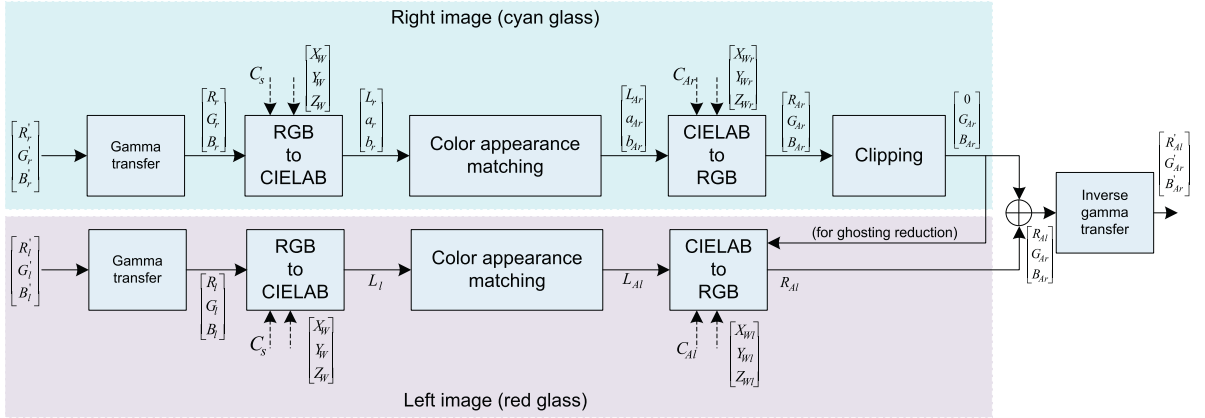
Fig. 2. Systematic framework of the proposed algorithm.
