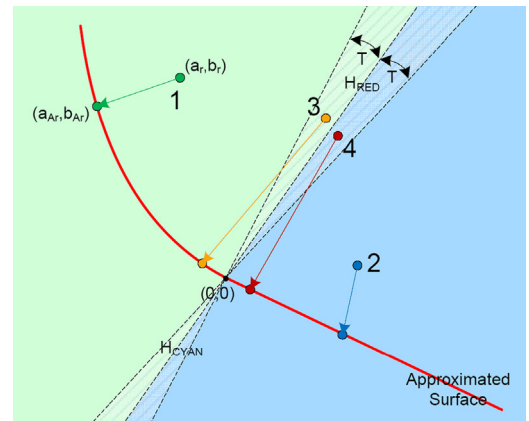
Fig. 4. The red line resembles the top view of the approximation surface as shown in Fig. 3(c). Examples 1–4 illustrate how Eqs. (10) and (11) project \{a_r, b_r\} to \{a_{Ar}, b_{Ar}\} in the CIELAB color space. Constant T is from Eq. (11).
