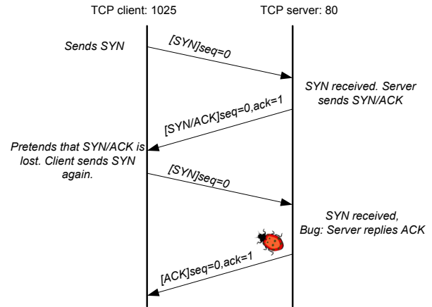
Figure 5. SYN packet loss.
