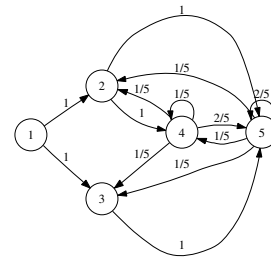
(c) Random Graph produced by our Model
