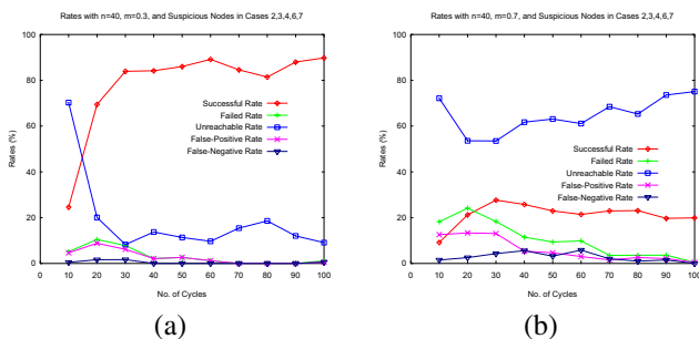
Figure 5. Rates with n=40 , r=100 , and Isolation of Suspicious Nodes in Cases 2,3,4,6,7 (a) m=0.3 (b) m=0.7
