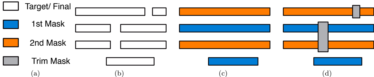
Figure 2. Process of LELEEC (a) Some labels. (b) Target features. (c) First and second mask patterns. (d) Trim mask, and final decomposition with no conflict.
