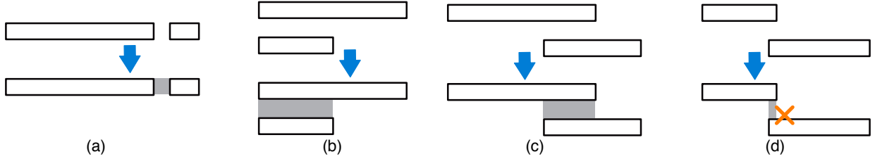
Figure 5. End-cut candidate generation for edge-edge type.
