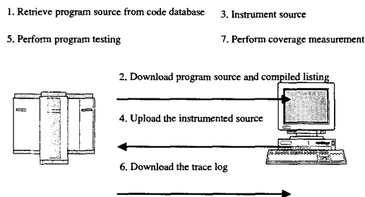
Figure 3. ATACOBOL Testing Setup
