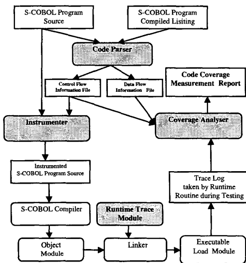
Figure 4. ATACOBOL Architecture
