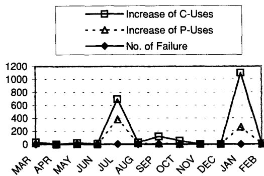
Figure 8. Number of Failure with C- and P-Uses Changes
