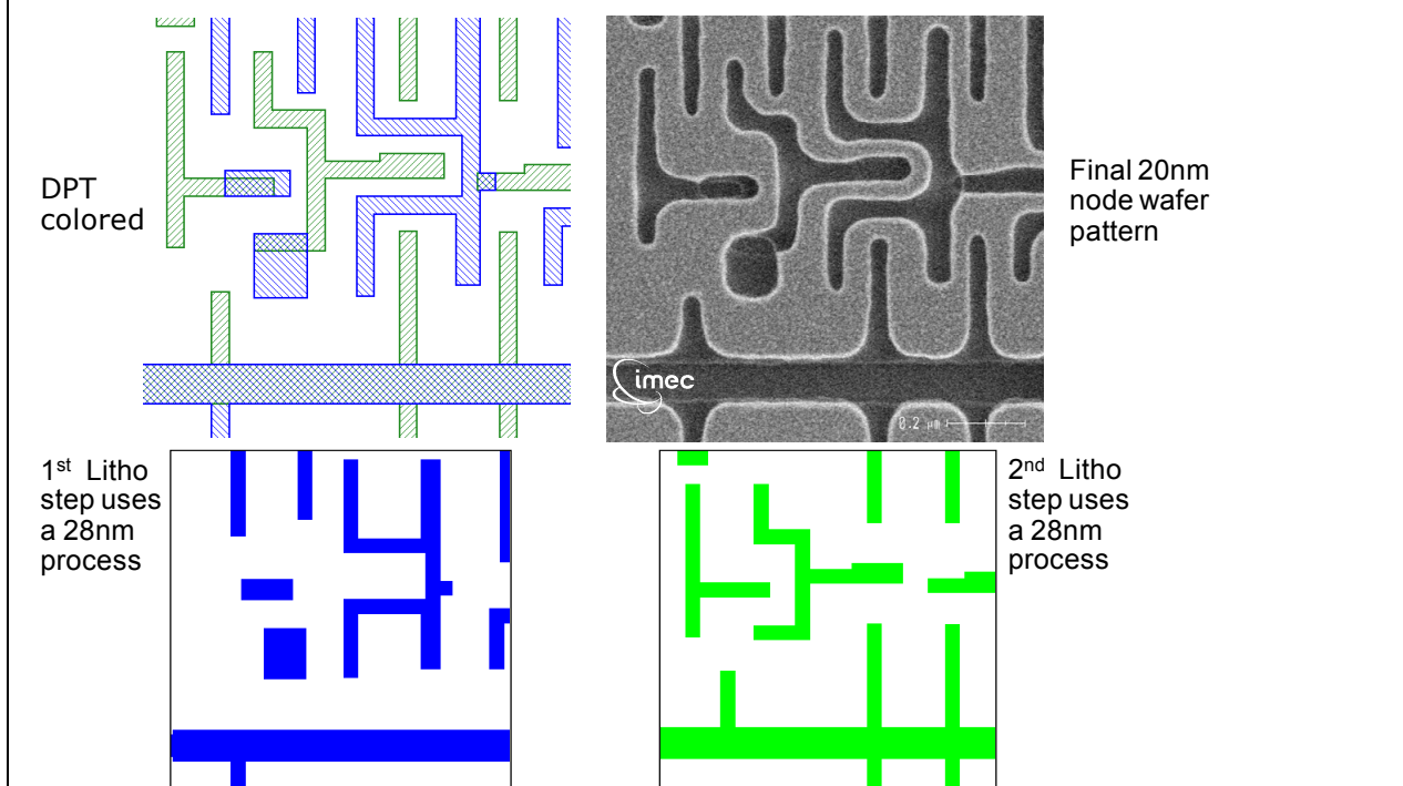
Figure 2. Example showing the flow of LELE DPT design decomposition and patterning. The metal layer design is decomposed into 2 masks (colors) then each is patterned with a ~28nm LE process. [2]
