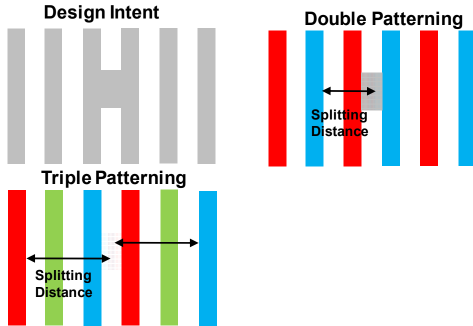
Figure 5. Examples of metal routing configuration in design and with double and triple patterning showing the large potential area shrink benefit of triple patterning for generally 1D features. [8]
