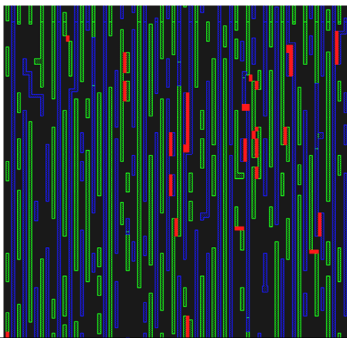
Figure 13. Example of a “poor man’s TPT” decomposition upon a 20nm DPT compliant routing layout shrunk ~30% to 14nm pitch. This method decomposes quickly to find conflicts which can be resolved by introducing a 3 rd mask color. However, color balancing is poor.
