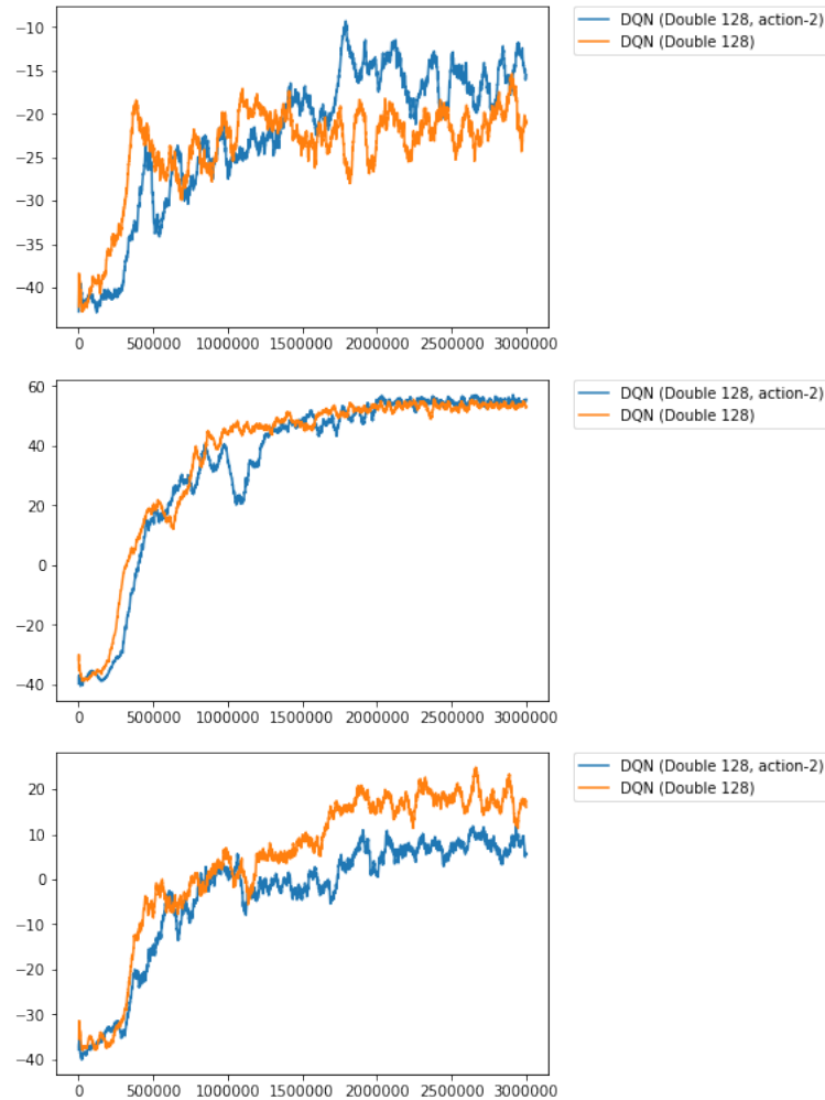
FIGURE 6.21: mean 100 episodic reward of DQN against in-game AI 0, 1 and 2.
