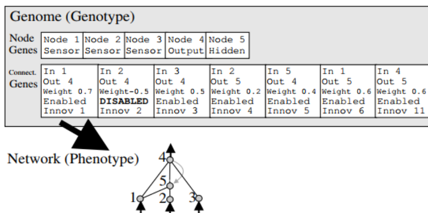
FIGURE 2.1: An example NEAT genome
