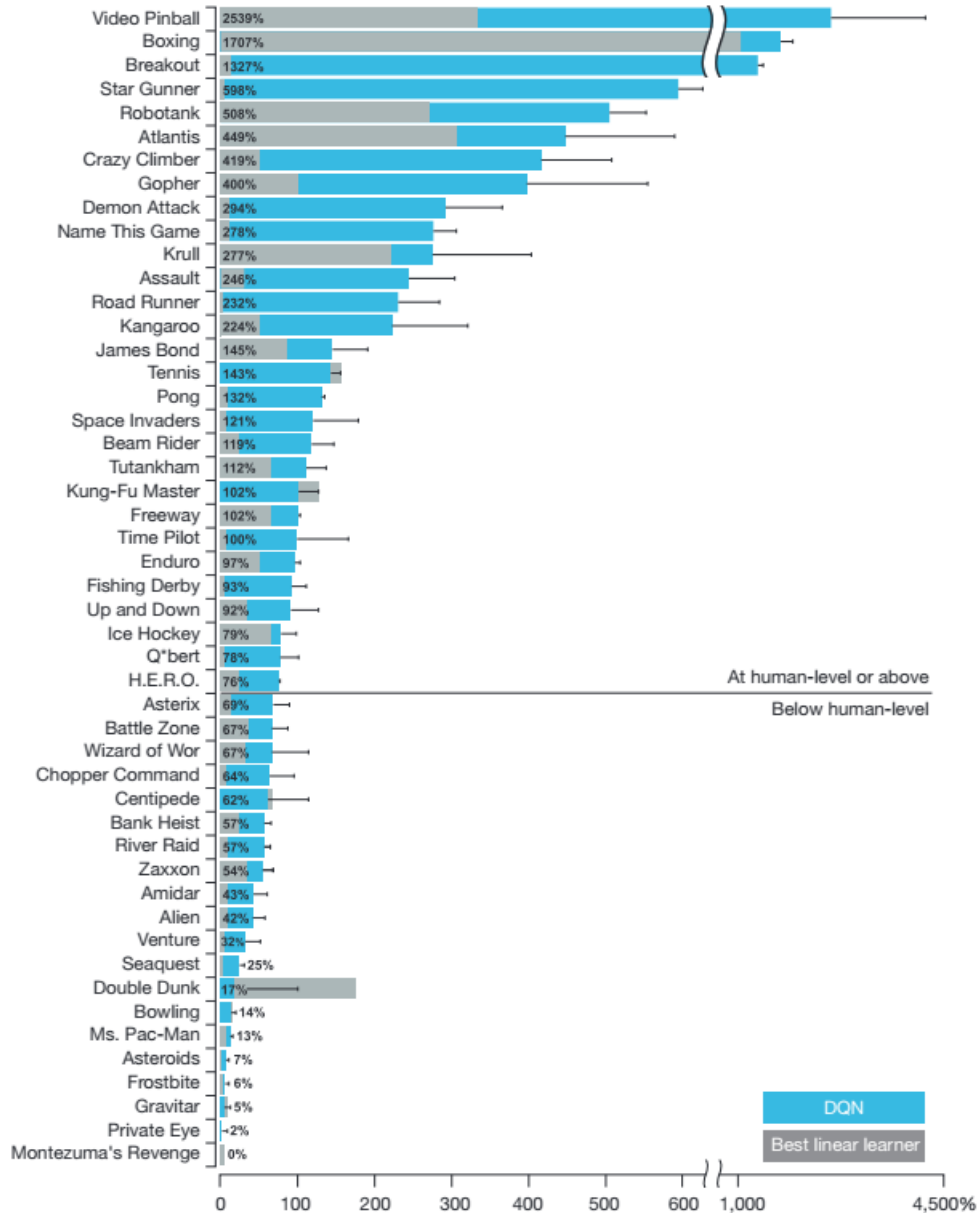
FIGURE 2.5: Normalized score achieved by DQN in different Atari 2600 games.
