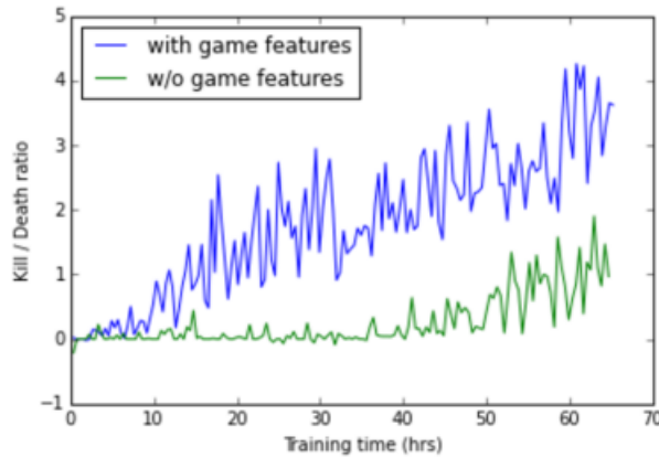
FIGURE 2.11: The kill-death ratio versus training hours of models trained with and without the game feature augmentation layers.
