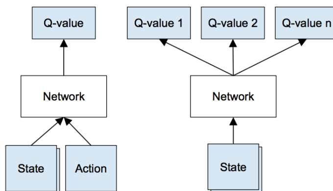
FIGURE 2.7: Two possible ways to approximate a Q-function. The right way is used in the paper.
