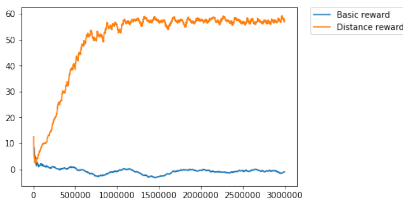
FIGURE 6.5: Mean 100 episodic reward of MLP-based DQN under different reward scheme.
