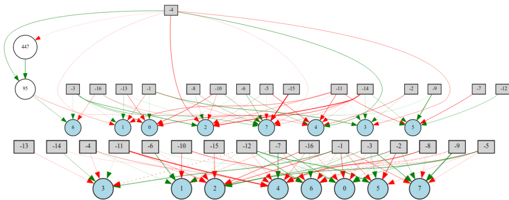
FIGURE 6.2: Two top 30th generation genome sampled from the result of setup D
