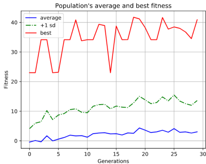
FIGURE 6.1: The maximum, average and standard deviation of fitness for each generation under setup D.
