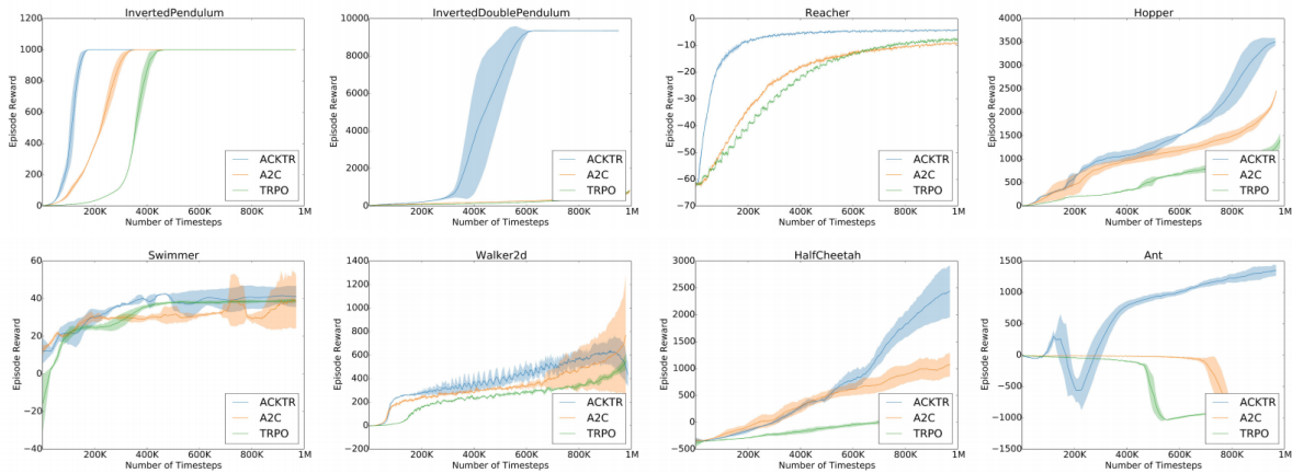
FIGURE 2.12: Performance of ACKTR compared to other state-of-the-art methods on MuJoCo benchmarks.
