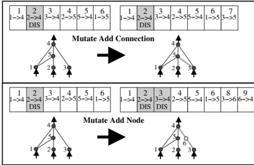
FIGURE 2.2: Illustration of types of NEAT mutation. The number written on top of each gene represent the innovation number generated during mutation.
