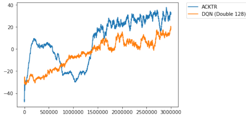
FIGURE 6.16: mean 100 episodic reward of ACKTR against random agent.
