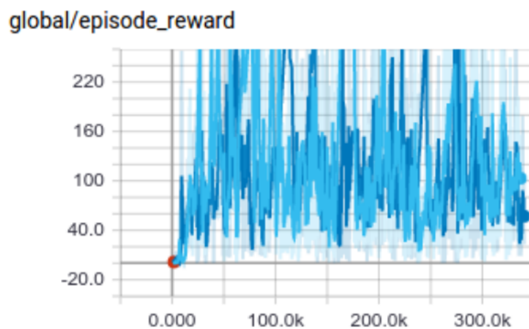
FIGURE 4.4: Training curve of A3C on slither.io. The two lines represent the episodic reward of two agents, other agents are removed for clarity.
