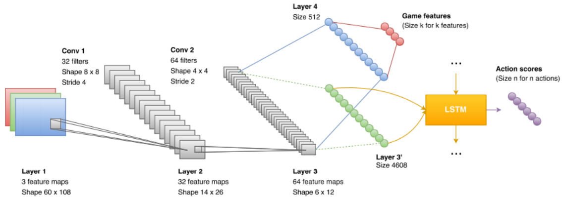
FIGURE 2.10: The network structure augmented with game feature layers.
