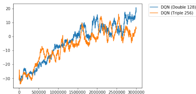
FIGURE 6.15: mean 100 episodic reward of DQN against random opponents.
