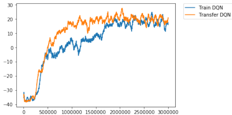
FIGURE 6.11: Transfer learning.
