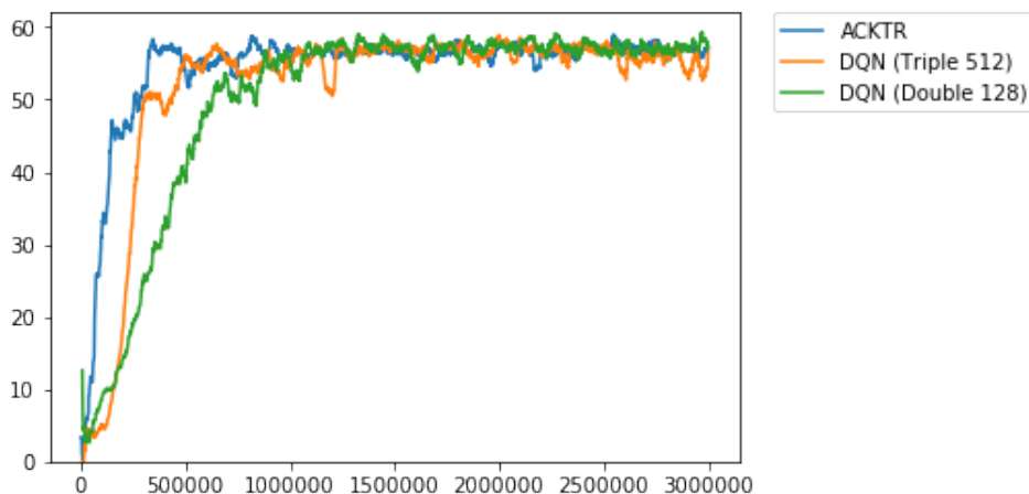
FIGURE 6.7: Mean 100 episodic reward of MLP-based ACKTR compare to MLP-based DQN.
