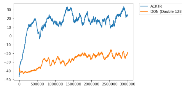
FIGURE 6.13: mean 100 episodic reward of ACKTR against in-game AI 0, comparing to DQN.
