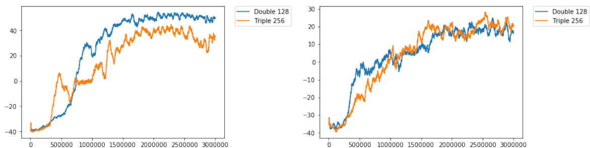
FIGURE 6.9: Mean 100 episodic reward of MLP-based DQN trained against in-game AI 1 and 2.
