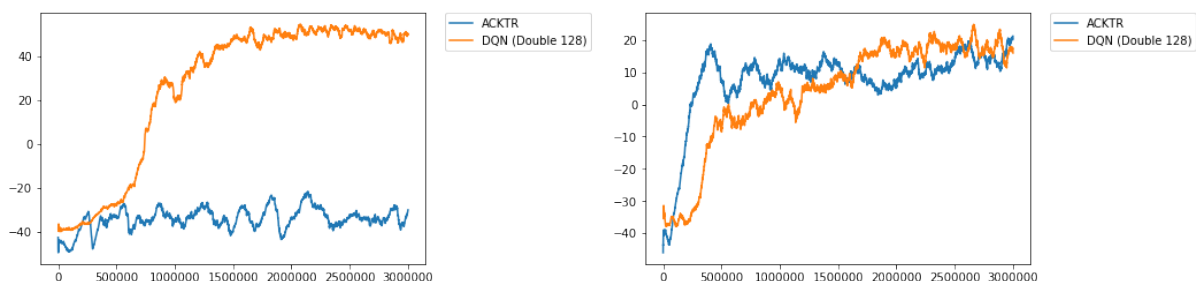
FIGURE 6.12: mean 100 episodic reward of ACKTR against in-game AI 1 and 2.
