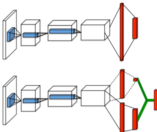
FIGURE 3.2: Comparing the structure of vanilla DQN (upper) and dueling network (lower).
