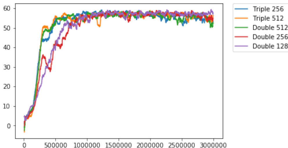
FIGURE 6.6: Mean 100 episodic reward of MLP-based DQN of different structures.
