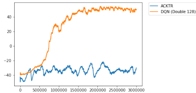
FIGURE 5.11: Mean 100 episodic reward.
