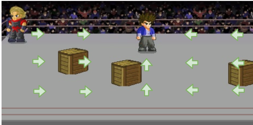
FIGURE 6.8: Green arrows represent the optimal policy when the agent is placed on that position.
