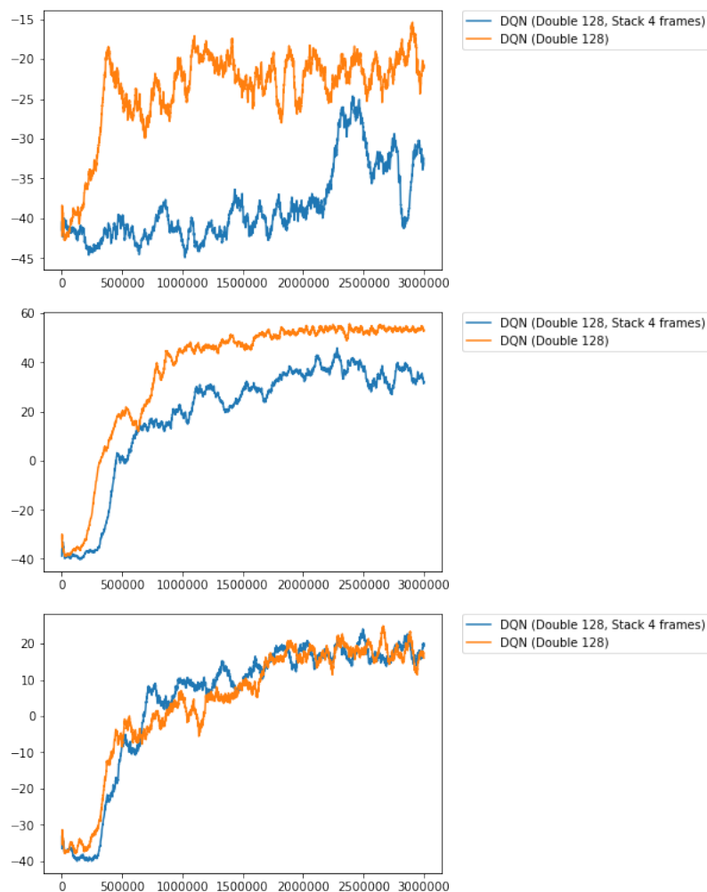
FIGURE 6.18: mean 100 episodic reward of DQN against in-game AI 0, 1 and 2.
