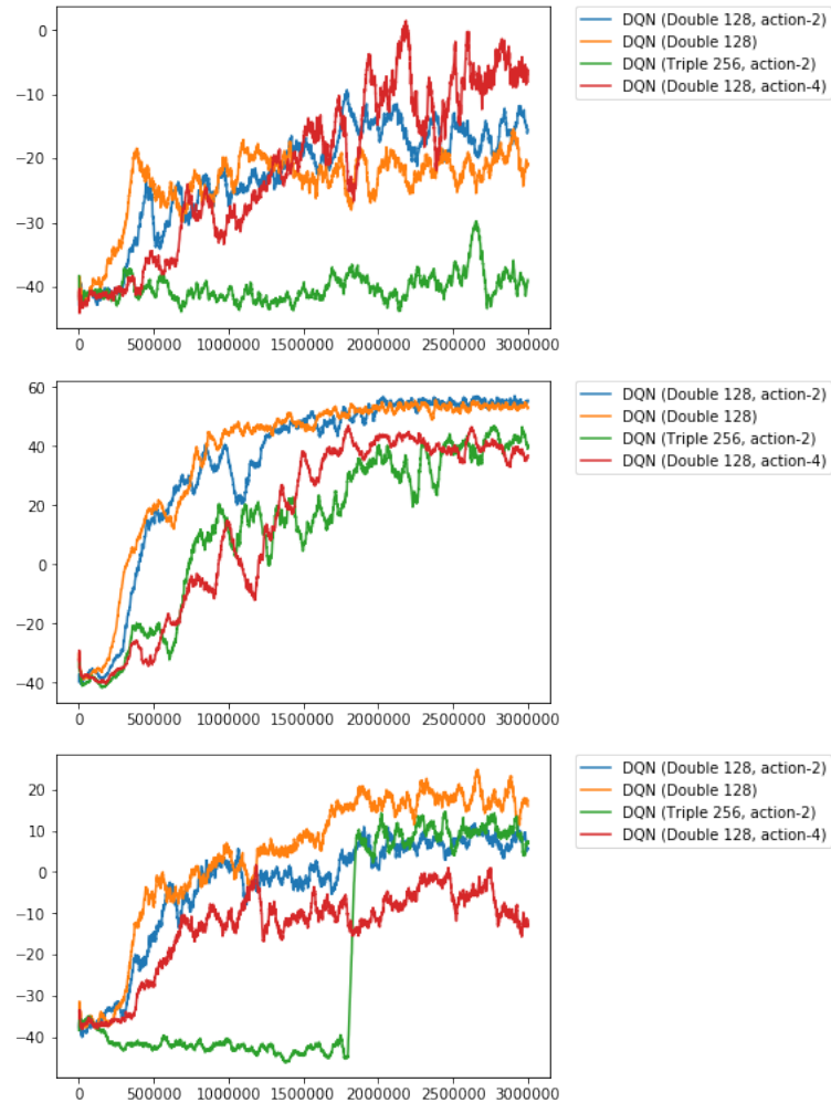
FIGURE 6.23: mean 100 episodic reward of DQN against in-game AI 0, 1 and 2.
