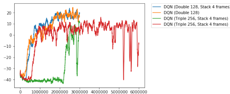
FIGURE 6.20: mean 100 episodic reward of DQN against in-game AI 2.
