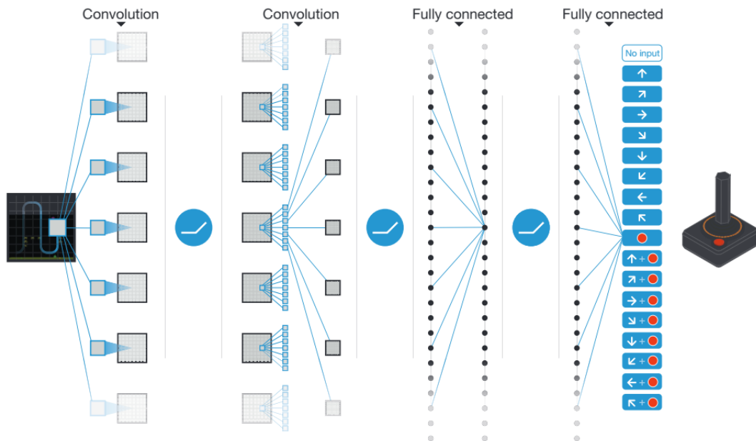
FIGURE 2.6: A high level description of general DQN structure.
