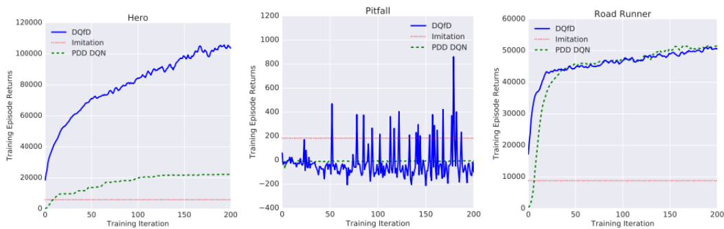
FIGURE 2.8: DQfD performance compared to pure imitation learning and DQN in three Atari games.
