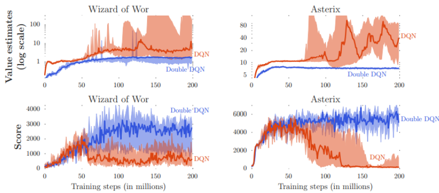
FIGURE 3.1: Averaged Q-values estimation and reward of vanilla DQN and Double DQN during training on two Atari games.
