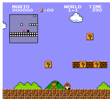
FIGURE 5.3: The state representation used by Seth Bling in his Mario NEAT project.
