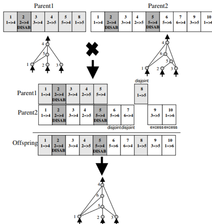
FIGURE 2.3: Illustration of NEAT crossover
