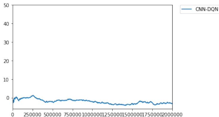
FIGURE 6.3: Mean 100 episode reward of setup P.
