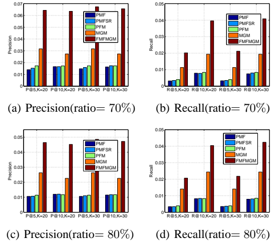
Figure 4: Performance Comparison
