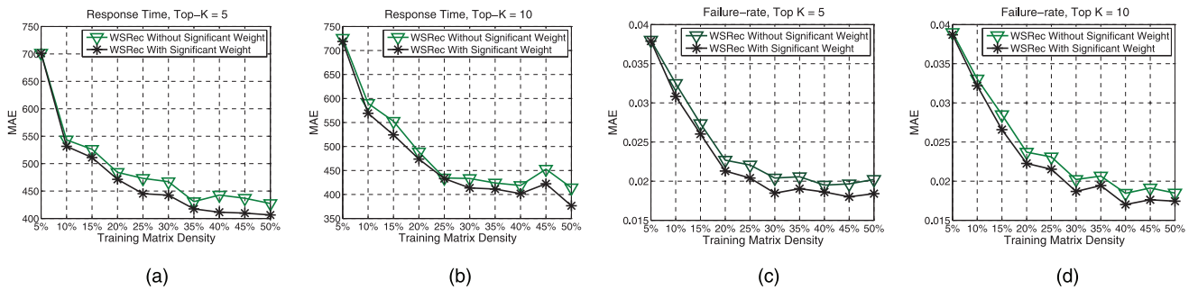
Fig. 5. Impact of the significance weight.
