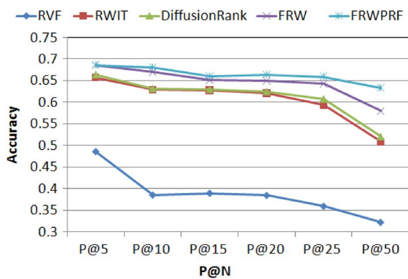
Fig. 6. P@N comparisons in CBIR.
