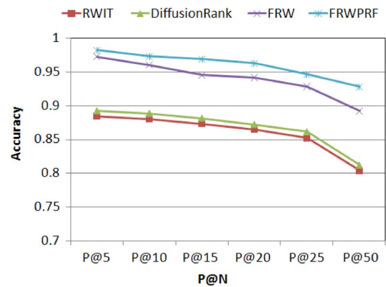
Fig. 10. P@N comparisons in TBIR.
