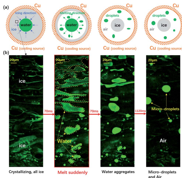
Fig. 1 The sudden melting event captured by confocal microscopy. The focal plane is right above the water–substrate interface. (a) The overall schematic illustration of the sudden melting event at the bottom substrate. The setup was a copper well with a diameter of 4 mm, which is cooled to below 0\text{ }^\circ\text{C} . The grey region indicates ice, the green region represents liquid water and the white region indicates air. (b) The real melting images recorded by confocal microscopy. In panel 1 the entire field of view is frozen (the bright region is due to the accumulation of fluorescent dye). In panel 2 melting occurs within 70 ms, replacing the ice with liquid water and a thin air gap with a thickness of 10 \mu\text{m} to 20 \mu\text{m} . In panels 3 and 4 the liquid water aggregates into circular micro-droplets. Also see Movie M1.†
