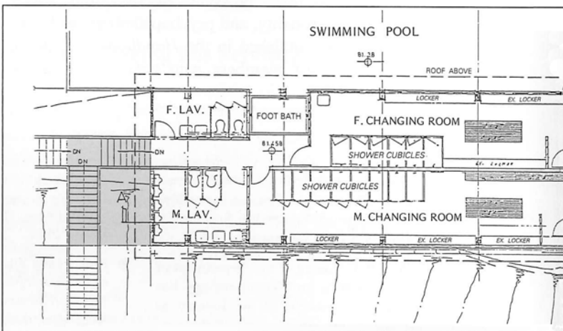
A plan of the expanded pool pavilion: the shaded areas mark the extensions already built or which are due to be completed.
