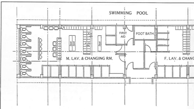
The lower storey of the expanded pavilion, with toilets and changing rooms for men and women at either ends
