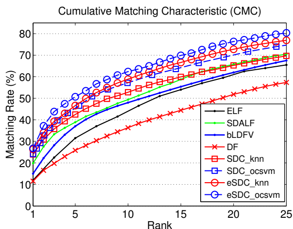
Figure 6. Performance on the VIPeR dataset. Our approach: SDC_knn and SDC_ocsvm. Our approach combined with wHSV and MSCR [10]: eSDC_knn and eSDC_ocsvm.
