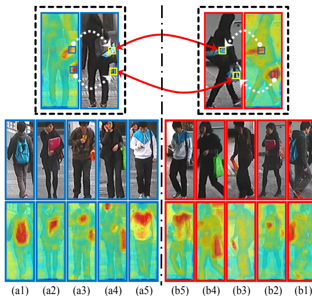
Figure 1. Examples of human image matching and saliency maps. Images on the left of the vertical dashed black line are from camera view A and those on the right are from camera view B . Upper part of the figure shows an example of matching based on dense correspondence and weighting with saliency values, and the lower part shows some pairs of images with their saliency maps.
