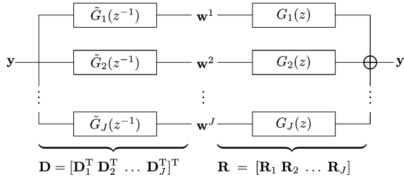
Fig. 3. Undecimated J -band analysis-synthesis filterbank.
