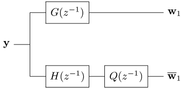
Fig. 4. GDC of the low-pass channel of an undecimated filterbank.
