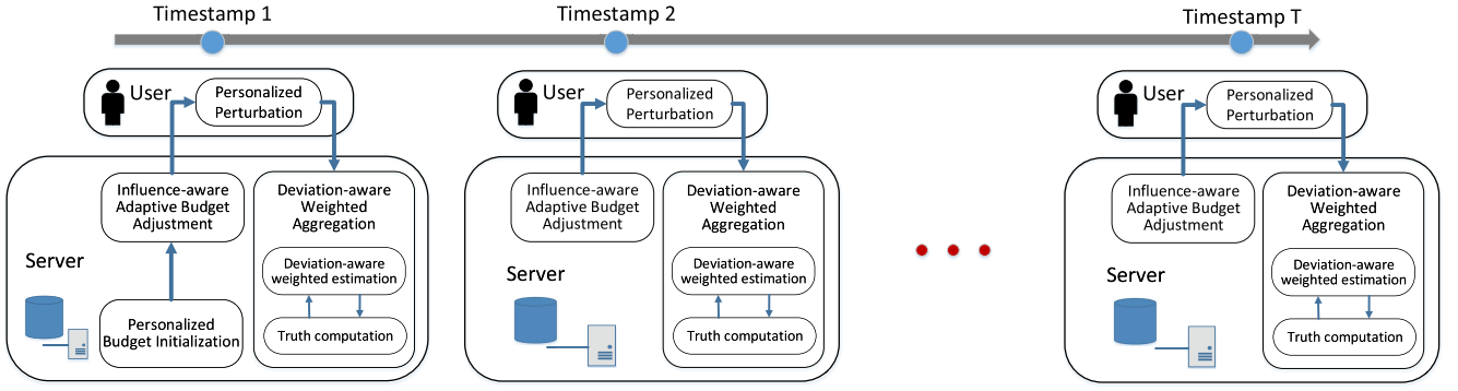
Fig. 2. Framework of the personalized privacy-preserving truth discovery mechanism.
