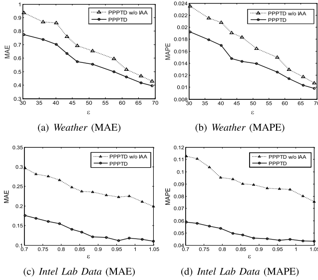
Fig. 8. Evaluation on IAA when \epsilon changes. (“w/o” stands for “without”).
