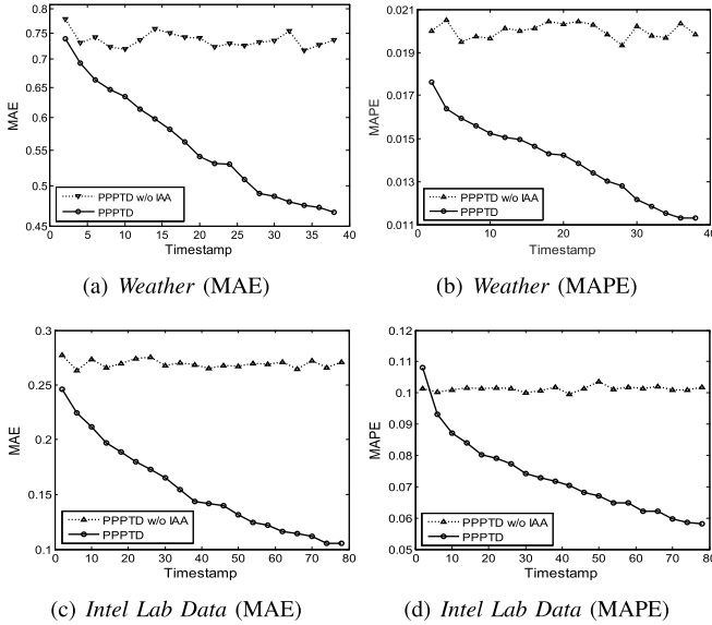
Fig. 9. Evaluation on IAA over time.
