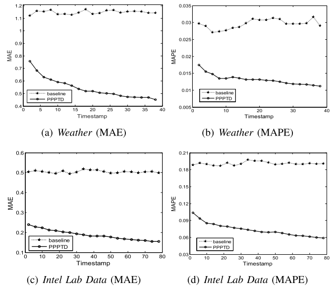
Fig. 12. Performance comparison of PPPTD and the baseline method.
