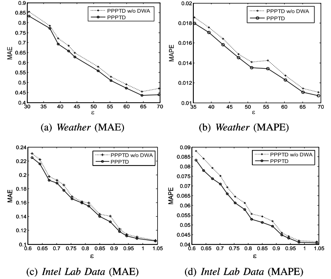
Fig. 11. Evaluation on DWA when \epsilon changes.
