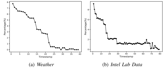
Fig. 10. Evaluation on the average percentage of users whose privacy budgets are updated per timestamp when (\pi, \rho) changes.
