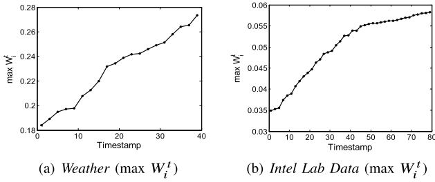
Fig. 3. The max value of W_i^t .
