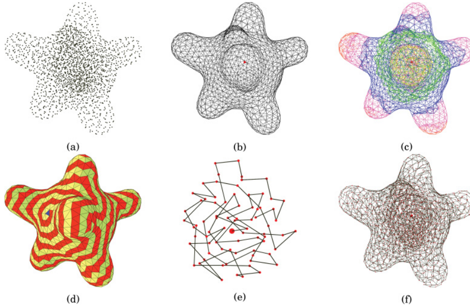
Fig. 2. Pipeline of the BLOW-UP algorithm. (a) A 3D volumetric network model with 2,290 nodes. (b) Boundary mesh; the center node is marked in red. (c) A series of connected and closed layers. (d) The spiral-like triangular strip (in red) on the outermost layer. (e) The segment of an SFC near the center node. (f) The constructed SFC of the network.
