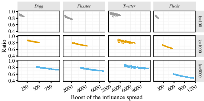
Fig. 11: Sandwich Approximation: \frac{\mu(B)}{\Delta_S(B)} (random seeds).
