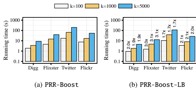
Fig. 10: Running time (random seeds).
