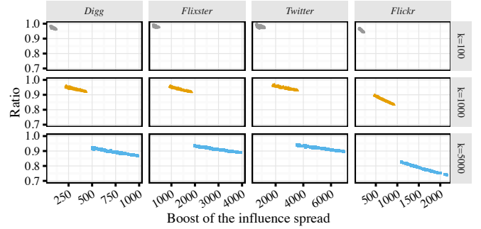
Fig. 6: Sandwich Approximation: \frac{\mu(B)}{\Delta_S(B)} (influential seeds).
