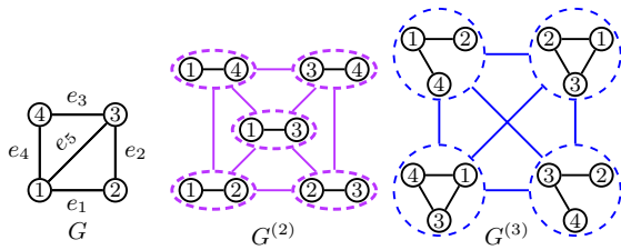
Figure 1: Original graph G and its 2 and 3-node subgraph relationship graph G^{(2)} and G^{(3)} .
