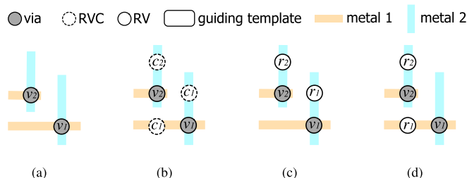
Fig. 1. (a) A layout; (b) Redundant via candidates; (c)(d) Two possible one redundant via insertion plans.
