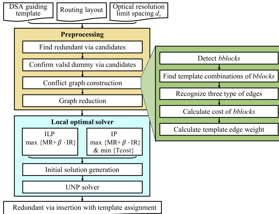
Fig. 7. Solution flow.
