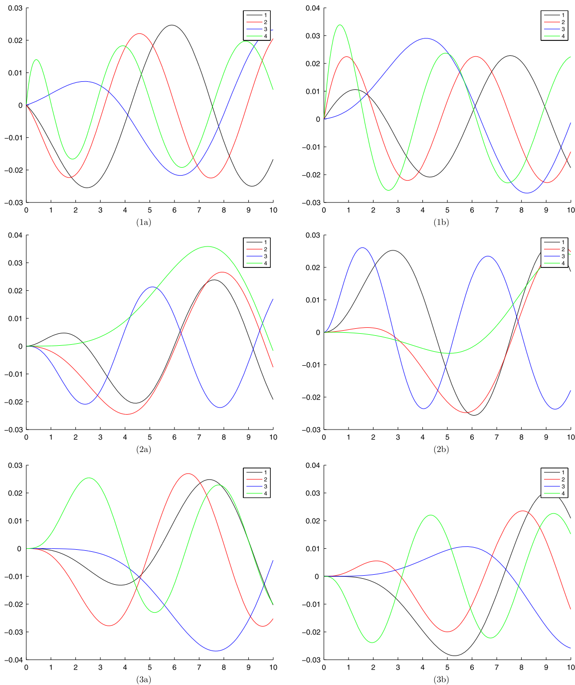
Fig. 2. Real and imaginary parts of the first 4 eigenfunctions of \tilde{K}_m^{(1)} , m = 1, 2, 3 . (1a) Real parts of eigenfunctions of \tilde{K}_1^{(1)} ; (1b) imaginary parts of eigenfunctions of \tilde{K}_1^{(1)} ; (2a) real parts of eigenfunctions of \tilde{K}_2^{(1)} , and so forth. (For interpretation of the references to color in this figure legend, the reader is referred to the web version of this article.)
