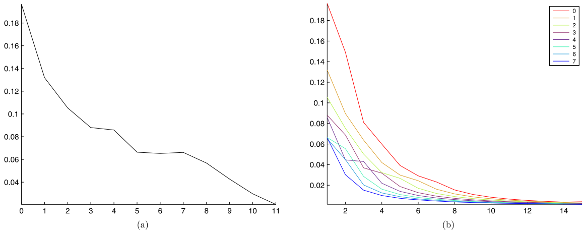
Fig. 1. (a) Spectral radius of \tilde{K}_m^{(1)} for m = 0, 1, \dots, 11 . (b) Norms of eigenvalues \lambda_{m,l} , l = 1, 2, \dots, 15 , for operators \tilde{K}_m^{(1)} , m = 0, 1, \dots, 7 , as in the legend. (For interpretation of the references to color in this figure legend, the reader is referred to the web version of this article.)
