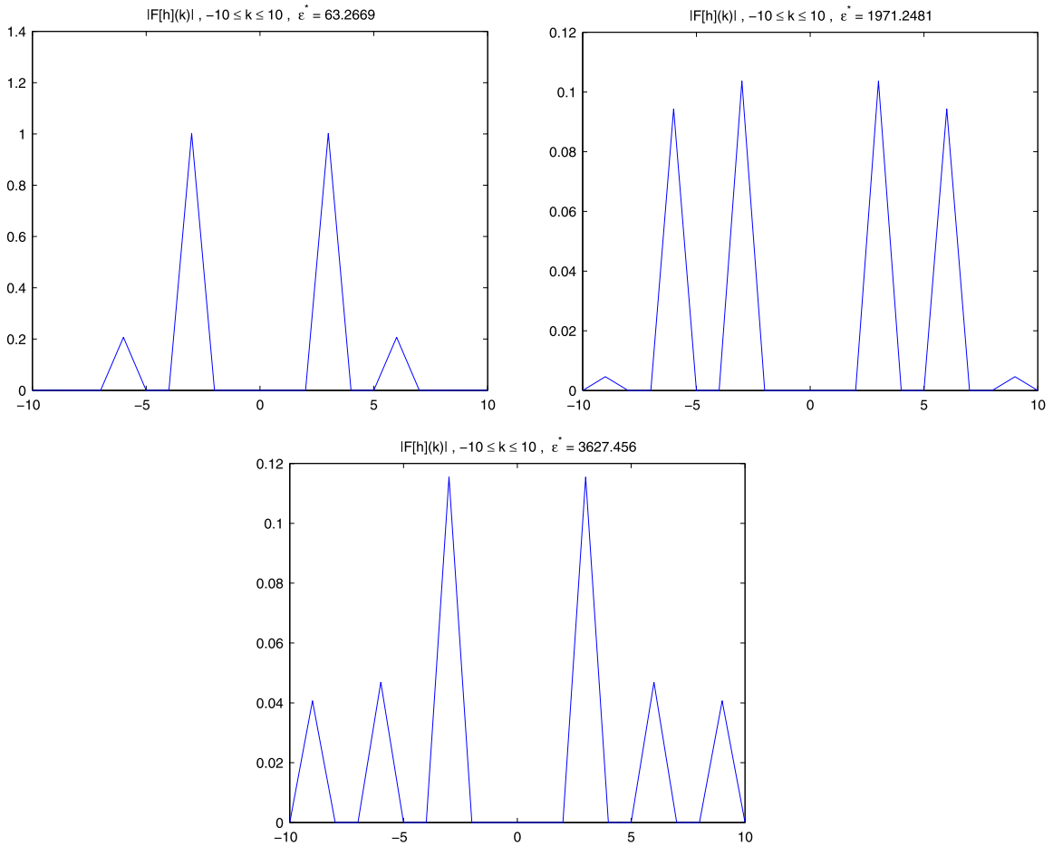
Fig. 6. Illustration of super-resolution in Example 1 : magnitude of recovered Fourier coefficients, \mathfrak{F}_\theta [h]^{\text{recovered}}(k) , -10 \leq k \leq 10 . Left: \epsilon^* = 63.2669 ; right: \epsilon^* = 1971.2481 ; bottom: \epsilon^* = 3627.456 .
