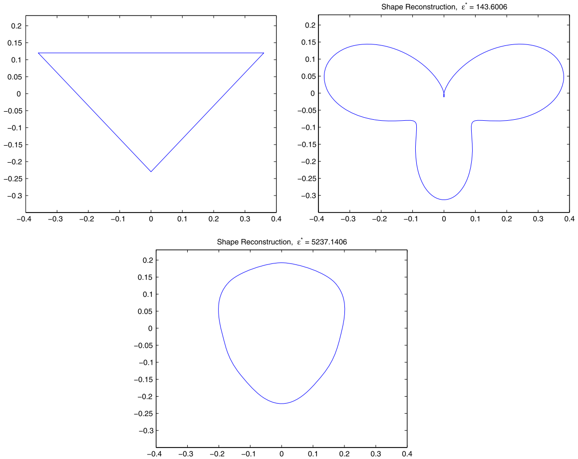
Fig. 12. Illustration of super-resolution in Example 2 : exact and recovered domains. Left: exact domain. Right: \varepsilon^* = 143.6006 ; bottom: \varepsilon^* = 5237.1406 .
