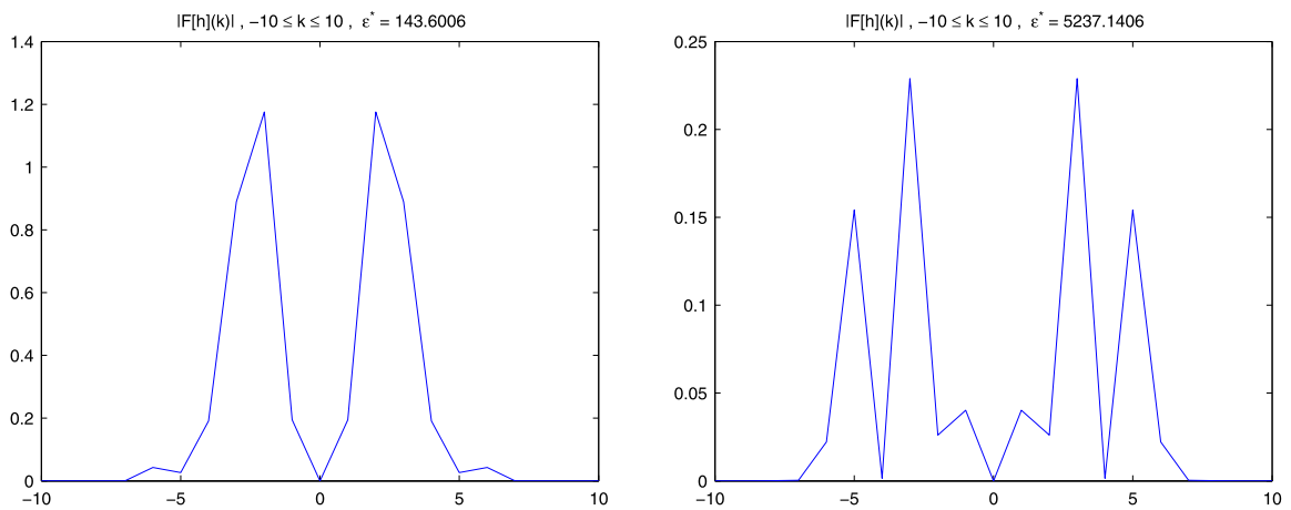
Fig. 11. Illustration of super-resolution in Example 2 : magnitude of recovered Fourier coefficients, \mathfrak{F}_\theta [h]^{\text{recovered}}(k) , -10 \leq k \leq 10 . Left: \epsilon^* = 143.6006 ; right: \epsilon^* = 5237.1406 .
