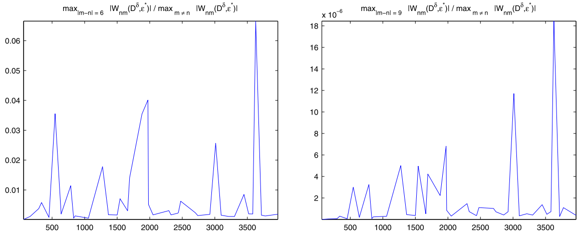
Fig. 4. Relative magnitudes of the scattering coefficients in Example 1. Left: the fraction of \max_{|m-n|=6} \{|W_{nm}(D^\delta, \epsilon^*)|\} / \max_{m \neq n} \{|W_{nm}(D^\delta, \epsilon^*)|\} , Right: the fraction of \max_{|m-n|=9} \{|W_{nm}(D^\delta, \epsilon^*)|\} / \max_{m \neq n} \{|W_{nm}(D^\delta, \epsilon^*)|\} .
