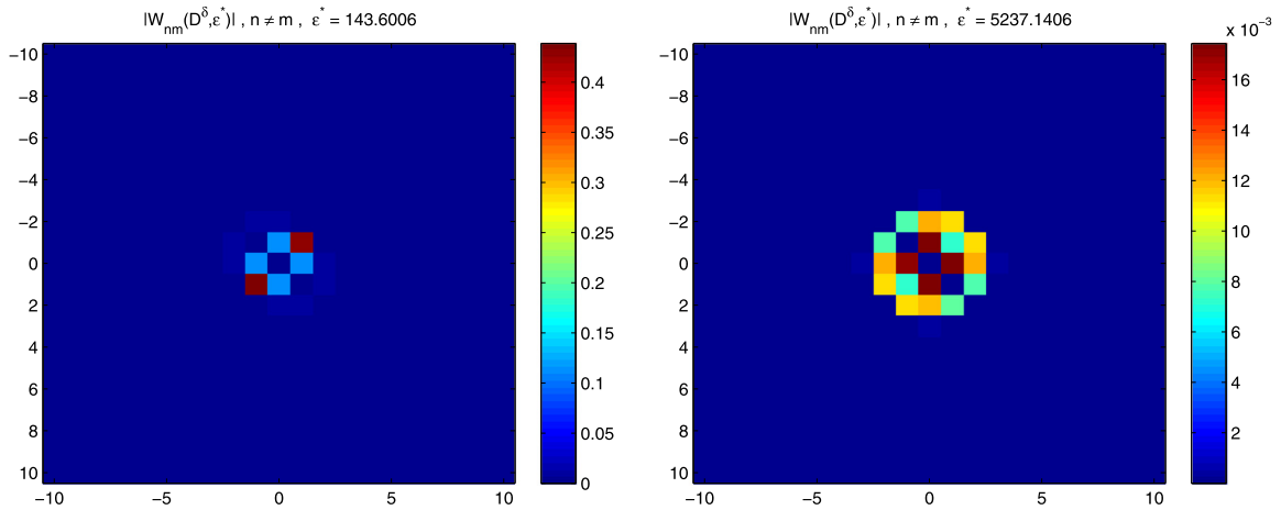
Fig. 10. Illustration of super-resolution in Example 2 : magnitude of scattering coefficients, |W_{nm}(D^\delta, \epsilon^*)| where -10 \leq m, n \leq 10 . Left: \epsilon^* = 143.6006 ; right: \epsilon^* = 5237.1406 .
