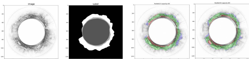
Fig 9. Sample of image in test set with corresponding label. Color in label from dark to bright
