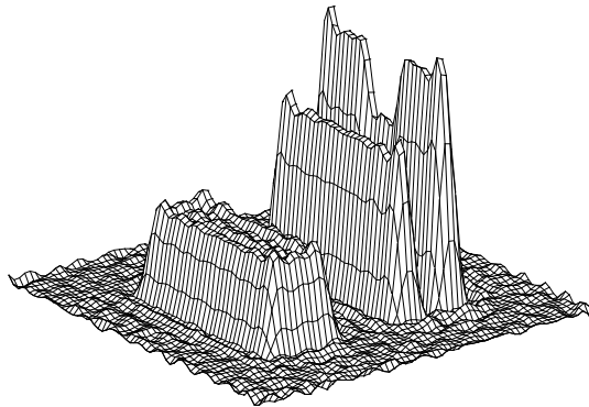
Figure 5b: Restoration using the Level-1 preconditioner (32 iterations).
