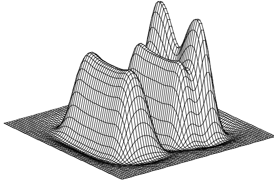
Figure 4a: Restoration after 2 iterations using no preconditioner.
