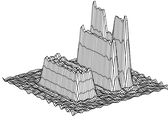
Figure 5a: Restoration using no preconditioner (108 iterations).
