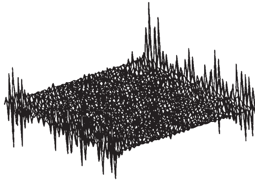
Figure 3: Restoration after 2 iterations with Level-1 preconditioner and no regularization.
