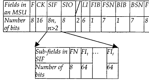
Fig. 2. MSU of CCS7. The SIF subfield embeds the surveillance information of all network components and branches. F : a marker with sequence "01 111 110" to signify the beginning and ending of an MSU; BSN : backward sequence number; BIB : backward indicator bit; FSN : forward sequence number; FIB : forward indicator bit. The BSN, BIB, FSN and FIB are designed for error correction, message sequence control, confirmation and re-transmission. LI : length indicator specifying the length of SIF. CK : error checking code; SIO : service indicator octet; FN : number of failed elements; FI j : information of the j th failed component.
