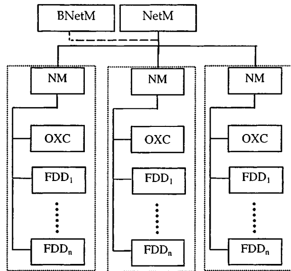
Fig. 1. Network management hierarchy. The WDM wavelength routing network is divided into different branches or links. All link components and subsystem will be monitored, and the switching node at which the fiber terminates will serve as the node manager. The health status will be sent to the node managers and then to the network manager through a separate independent signaling network. NetM—network manager, BnetM—backup network manager, NM—node manager, FDD—fault detection device, and OXC—optical cross-connect.
