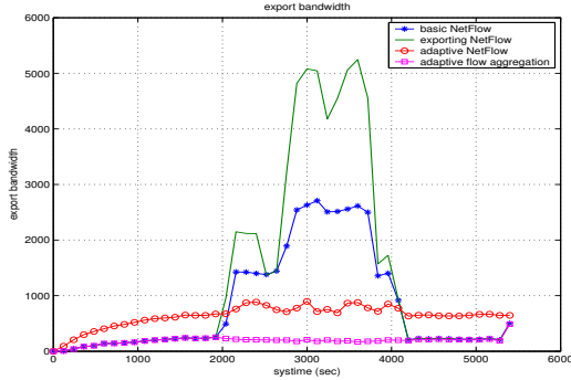
Fig. 7. export bandwidth for different solutions
