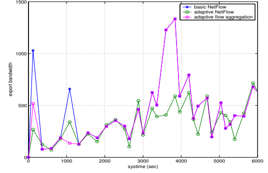
Fig. 12. export bandwidth of adaptive NetFlow & adaptive flow aggregation
