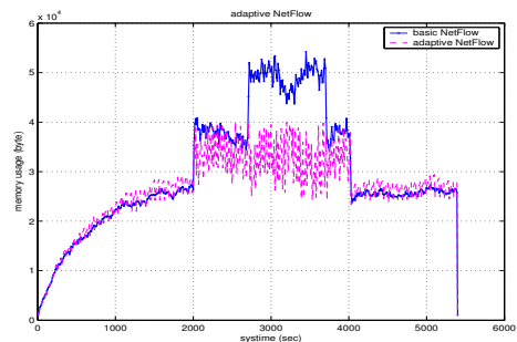
Fig. 5. memory usage for adaptive NetFlow
