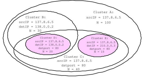
Fig. 2. three levels of cluster
