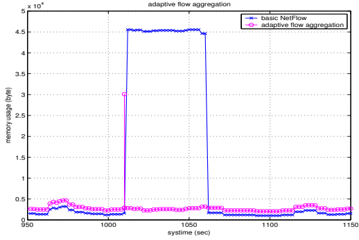
Fig. 14. memory usage of adaptive flow aggregation under DoS attack
