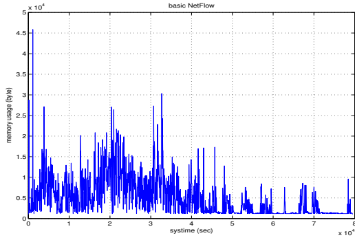
Fig. 9. memory usage of basic NetFlow
