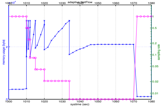
Fig. 13. memory usage of adaptive NetFlow under DoS attack
