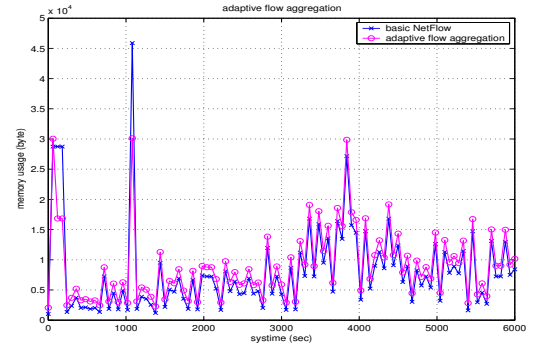
Fig. 11. memory usage of adaptive flow aggregation
