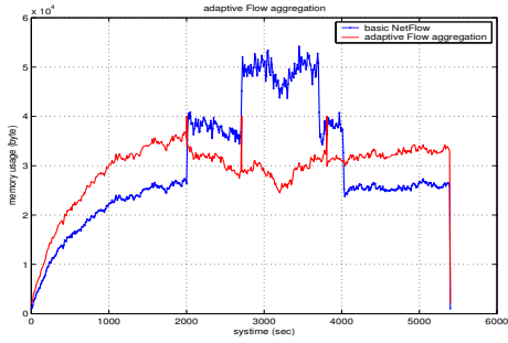
Fig. 6. memory usage for adaptive flow aggregation
