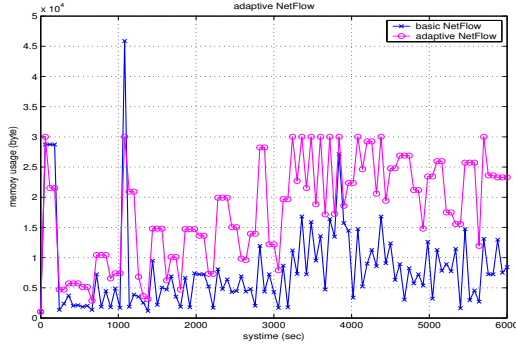
Fig. 10. memory usage of adaptive NetFlow
