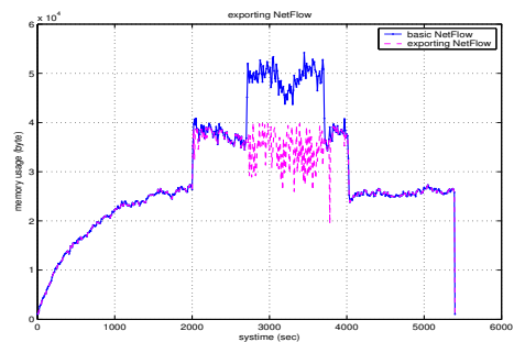
Fig. 4. memory usage for exporting NetFlow
