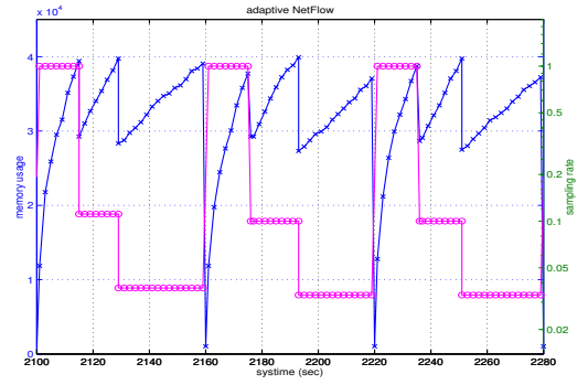
Fig. 8. memory usage and sampling rate in several measurement bins
