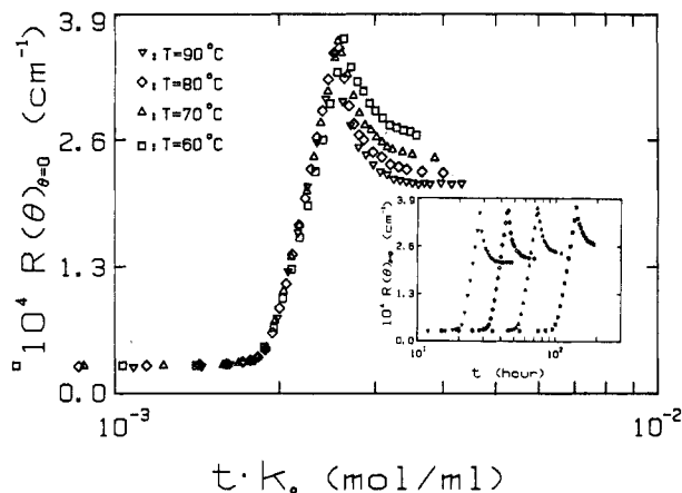
Figure 3. R_{vv}(\theta)_{\theta=0} versus scaled reaction time, k_0 t (in units of mol/mL), at four different reaction temperatures, 60, 70, 80, and 90 °C. The molar ratio of DGEb:CH:CA = 1:2:0.001. Inset: Unscaled R_{vv}(\theta)_{\theta=0} versus reaction time t (in units of hours).
