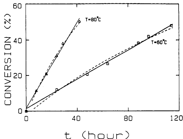
Figure 2. Anhydride (CH) conversion ( ([CH]_0 - [CH]_t)/[CH]_0 , %) versus reaction time t at two different temperatures, 60 and 80 °C. The molar ratio of DGEb:CH:CA = 1:2:0.001. Solid line for zeroth-order fitting. Dot line for second-order fitting.
