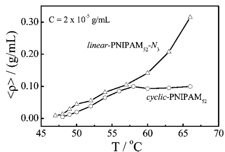
Figure 5. Temperature dependence of average chain density, \langle \rho \rangle , of PNIPAM mesoglobules formed in a slow heating process, where \langle \rho \rangle is defined as M_w / N_A [(4/3)\pi \langle R_h \rangle^3] .
