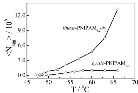
Figure 2. Temperature dependence of average aggregation number, \langle N_{\text{agg}} \rangle , of mesoglobules of cyclic -PNIPAM 52 and linear -PNIPAM 52 -N 3 formed during a slow heating process, where \langle N_{\text{agg}} \rangle = M_{w,\text{agg}}/M_{w,\text{chain}} with M_{w,\text{agg}} and M_{w,\text{chain}} the weight-average molar masses of the aggregates and the chains, respectively. Each data point was obtained after the temperature equilibrium was reached.
