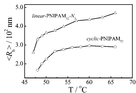
Figure 3. Temperature dependence of average hydrodynamic radius, \langle R_h \rangle , of mesoglobules of cyclic -PNIPAM 52 and linear -PNIPAM 52 -N 3 formed during a slow heating process. Each data point was obtained after the temperature equilibrium was reached.
