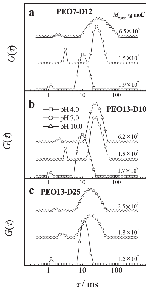
Figure 1. pH dependence of characteristic relaxation time distributions and corresponding apparent molecular weight of associates: (a) PAA- g -PEO-7- g -dodecyl-12; (b) PAA- g -PEO-13- g -dodecyl-10; (c) PAA- g -PEO-13- g -dodecyl-25 aqueous solutions at 20 °C. C_{\text{polymer}} = 2.7 \times 10^{-4} \text{g mL}^{-1} , C_{\text{NaCl}} = 0.025 M.
