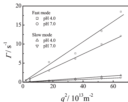
Figure 2. Scattering vector ( q ) dependence of average characteristic relaxation rate ( \Gamma ) of fast and slow relaxation modes for PAA- g -PEO-13- g -dodecyl-25 aqueous solutions with pH 4.0 and 7.0, 20 °C, C_{\text{polymer}} = 2.7 \times 10^{-4} \text{g mL}^{-1} , and C_{\text{NaCl}} = 0.025 M.
