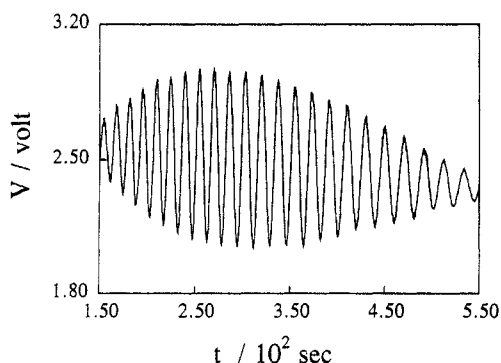
Figure 3. Part of typical voltage signal observed in the gel swelling process, where V is proportional to I in eq 9 (see text for details). The gel-swelling temperature is 29 °C, the initial gelatin concentration is 10%, and the initial film thickness is 60 \mu\text{m} .
