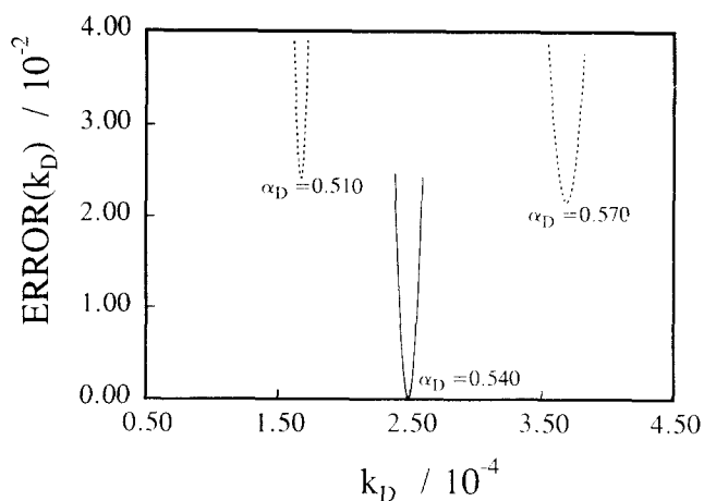
Figure 5 Typical plots of ERROR(k_D) versus k_D for different values of \alpha_D . The overall minimum value of ERROR(k_D) corresponds to \alpha_D = 0.540 and k_D = 2.49 \times 10^{-4}
