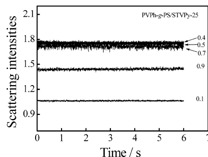
Figure 5. Time dependence of the scattering light intensities upon stopped-flow mixing PVPh- g -PS and STVPy-25 solutions in THF at different weight fractions of PVPh- g -PS; the total polymer concentration after mixing is 1.0 \times 10^{-4} g/mL.
