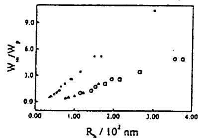
Figure 7. Typical plot of W_m/W_s versus R for dispersions obtained by emulsion polymerization of styrene in the presence of the short PEO chain as a stabilizer.
