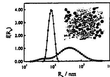
Figure 2. Comparison of the hydrodynamic radius distribution ( f(R_h) ) of PS nanoparticles prepared with (the sharp peak, while the insert is a TEM photo) and without microwave irradiation.
