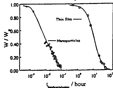
Figure 9. Comparison of biodegradation of a PCL thin film and nanoparticles under the same enzyme concentration.
