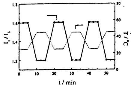
Figure 10. Temperature dependence of the fluorescence intensity ratio of pyrene in the presence of the core-shell PNIPAM-g-PEO nanoparticles.
