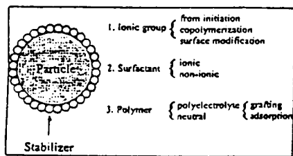
Figure 5. Schematic representation of stabilization of polymeric nanoparticles where the surface area per stabilizer is a constant for a given dispersion.
