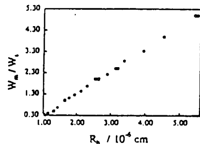
Figure 6. A typical plot of W_m/W_s versus R for the emulsion polymerization of styrene in the presence of CTAB as a stabilizer and AIBN as an initiator.
