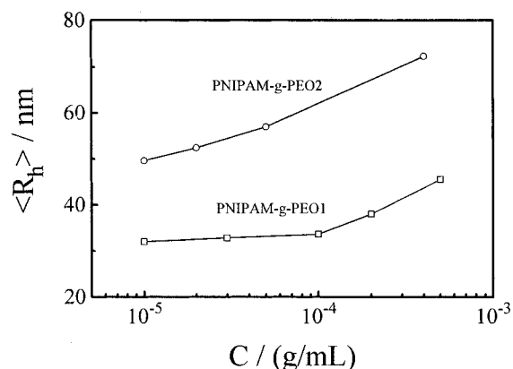
Figure 9. Comparison of the average hydrodynamic radius ( \langle R_h \rangle ) of the PNIPAM- g -PEO1 and PNIPAM- g -PEO2 nanoparticles formed with different initial polymer concentrations in the step-by-step slow heating from 25 to 45 °C.
