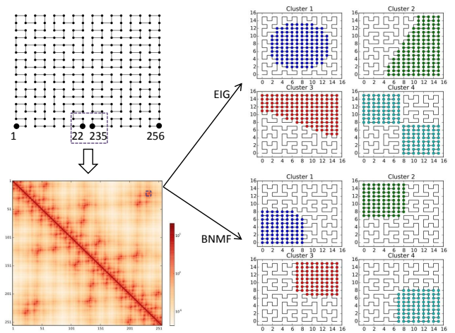
Fig. 2. Comparison between eigenvalue decomposition and BNMF based on a space-filling curve. A Hilbert curve is used to generate an artificial 2D chromosome and a corresponding synthetic contact map. The contact map is decomposed by eigenvalue decomposition (EIG) and BNMF. In both cases, four clusters are obtained by grouping the points with the highest coefficients along the eigenvectors or affinity values to the clusters. A region with long-range contacts, including points 22 and 235, is highlighted in the Hilbert curve, the heat map, and cluster 4 produced by BNMF.
