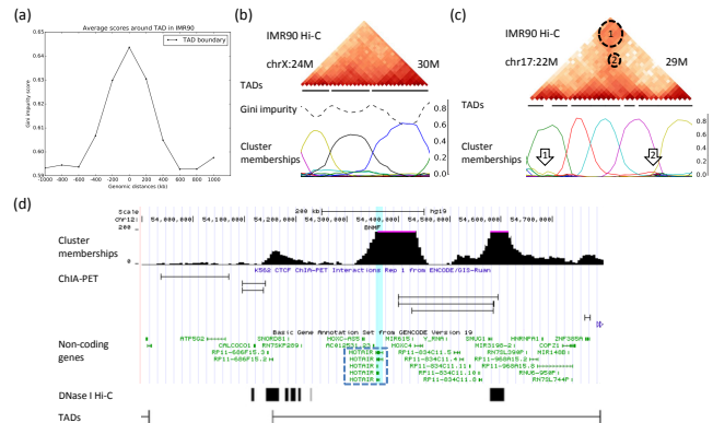
Fig. 4. Relationships between BNMF clusters and TADs. (a) Bins around TAD boundaries have increased Gini impurity scores, indicating that they are also at the boundaries of BNMF clusters. (b) An example showing a simple case in which each TAD corresponds to exactly one BNMF cluster. In the cluster affinity panel, each color represents a different cluster. (c) A more complex example showing that some TADs contain multiple clusters, and some long-range DNA contacts across multiple TADs (circles 1 and 2) appear as small peaks of cluster affinity values (marked by arrows 1 and 2). (d) An example showing a BNMF cluster with almost the same boundaries with a TAD, but the affinity values further show the long-range contacts between the HOTAIR gene and two distal regions that have been independently shown by ChIA-PET or DNase I Hi-C.
