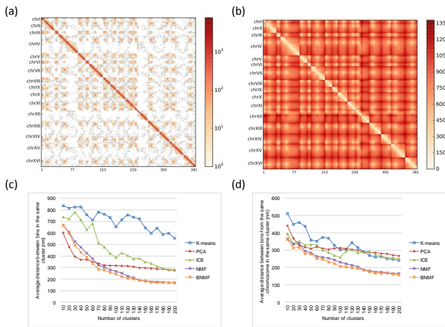
Fig. 3. Comparison between five different clustering methods based on the noisy synthetic yeast Hi-C contact map. (a) The contact map obtained from 3,000 simulated yeast genome structures with random biases added to each bin. (b) The corresponding average Euclidean distances between different bins in the 3,000 structures. (c) The average distance between bins in the same cluster. (d) The average distance between bins in the same cluster, considering only bin pairs from the same chromosome.
