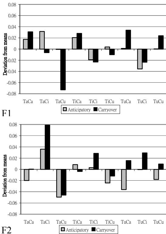
Fig. 2 Carryover vs anticipatory coarticulation for different Target and Context combinations at vowel edges for F1 (upper panel) and F2 (lower panel) pooled across Language and Stress. “T”: target vowel; “C”: context vowel.
