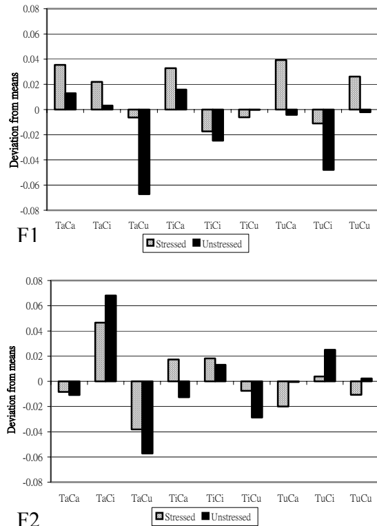
Fig. 1 Coarticulatory effects of Stress at vowel edges on F1 (upper panel) and F2 (lower panel), for different Target and Context combinations pooled across Language and Direction. "T": target vowel; "C": context vowel.
