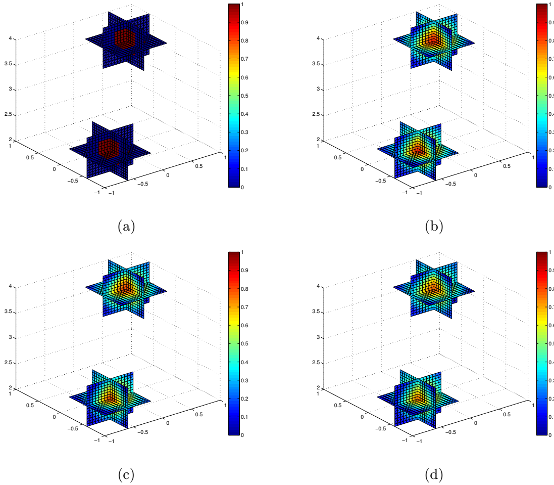
Figure 5: Exact contrast values q(x) (a), and distributions of the index function I(x) with 10% noise (b), 20% noise (c) and 30% noise (d) for Example 2.
