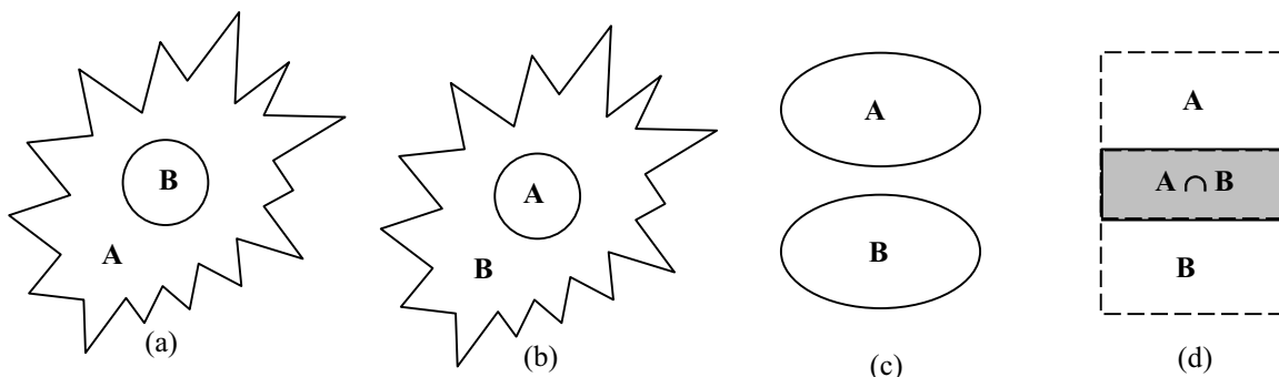
Figure 2. A is the principal subspace of S_w , B is the principal subspace of S_b , and \mathbf{A} \cup \mathbf{B} is the whole face space. In case (a), \mathbf{B} \subseteq \mathbf{A} , LDA in the principal space of S_w can keep all the discriminative information. In case (b), \mathbf{A} \subseteq \mathbf{B} , direct LDA can keep all the discriminative information. In case (c), \mathbf{A} \cap \mathbf{B} = \phi , LDA in the null space of S_w can keep all the discriminative information. In case (d), A and B are only partially intersect, and so discriminative information in data space will definitely be lost in conventional LDA approaches.
