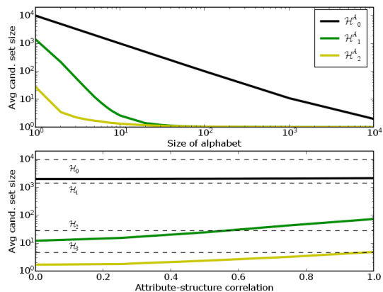
Figure 7: Effect of attribute knowledge on re-identification measured by average size of candidate sets. Top: attributes are sampled independently ( p = 0 ) from an alphabet of varying size. Bottom: attribute-structure correlation p varies while alphabet size is fixed at five. The dashed lines show candidate set sizes under \mathcal{H}_i (no attribute knowledge).
