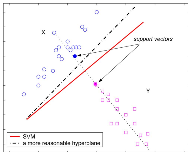
Fig. 1. Decision hyperplane with considerations of both local and global information.
