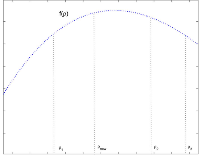
Fig. 4. Three-point pattern and quadratic line search method. A \rho_{\text{new}} is obtained and a new three-point pattern is constructed by \rho_{\text{new}} and two of \rho_1, \rho_2 , and \rho_3 .
