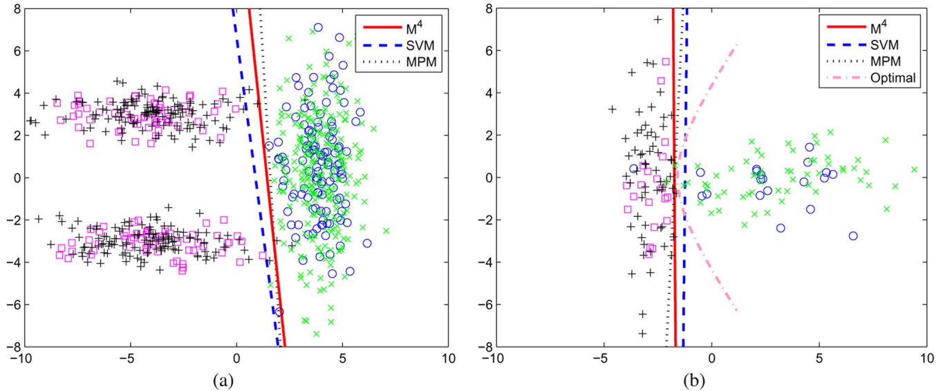
Fig. 6. Third and fourth synthetic toy examples to illustrate M^4 . Training (test) data, consisting of 120 (250) data points in (a) and 20 (60) in (b) for each class are presented as \circ 's ( \times 's) and \square 's ( + 's) for x and y , respectively. (a) Demonstration of M^4 performing better in a mixture of Gaussian data than SVM. (b) M^4 achieves the suitable decision boundary, which considers data both locally and globally.
