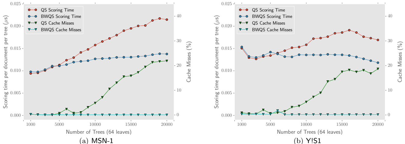
Figure 4: Per-tree per-document scoring time in \mu\text{s} and percentage of cache misses of QS and BWQS on MSN-1 (left) and Y!S1 (right) with 64-leaves \lambda -MART models.
