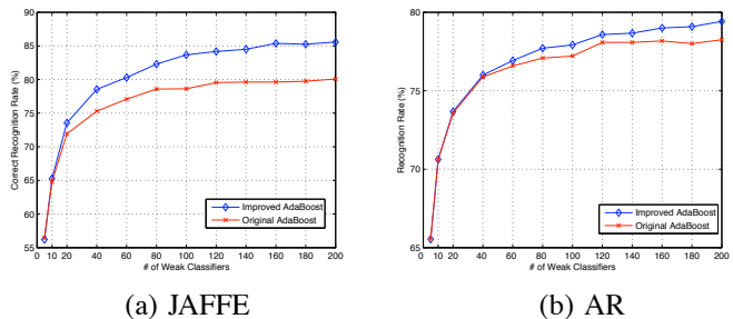
Fig. 3. Performance evaluation for the original AdaBoost algorithm and our improved AdaBoost algorithm.
