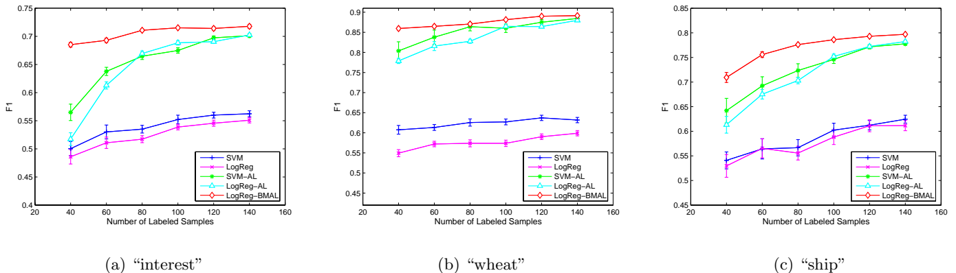
Figure 3: Experimental results of F1 performance on the “interest”, “wheat” and “ship” categories
