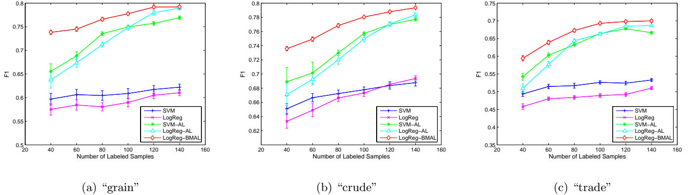
Figure 2: Experimental results of F1 performance on the “grain”, “crude” and “trade” categories
