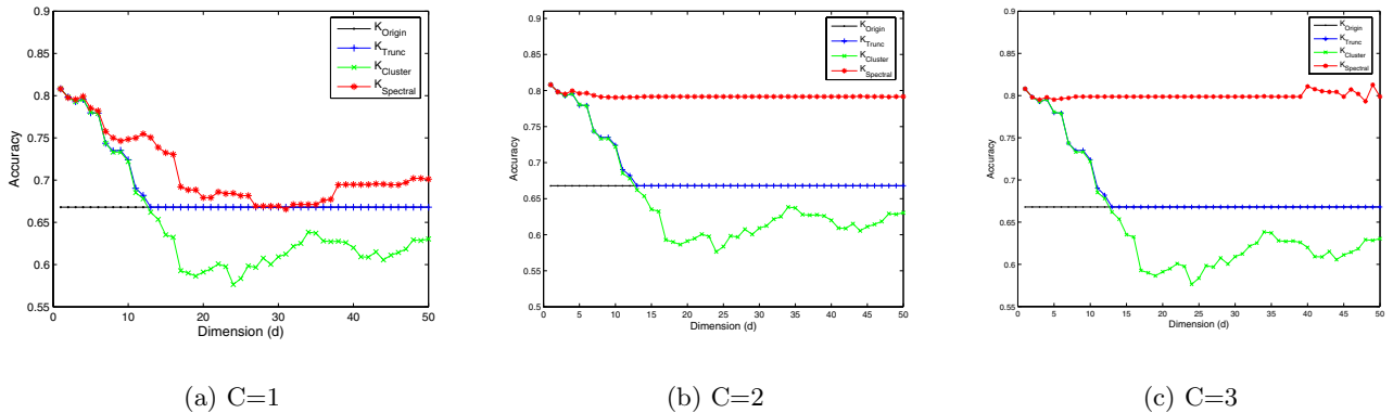
Figure 5: Classification performance of semi-supervised kernels with different decay factors on the Heart dataset. The initial kernel is a linear kernel and the number of labeled data is 20.
