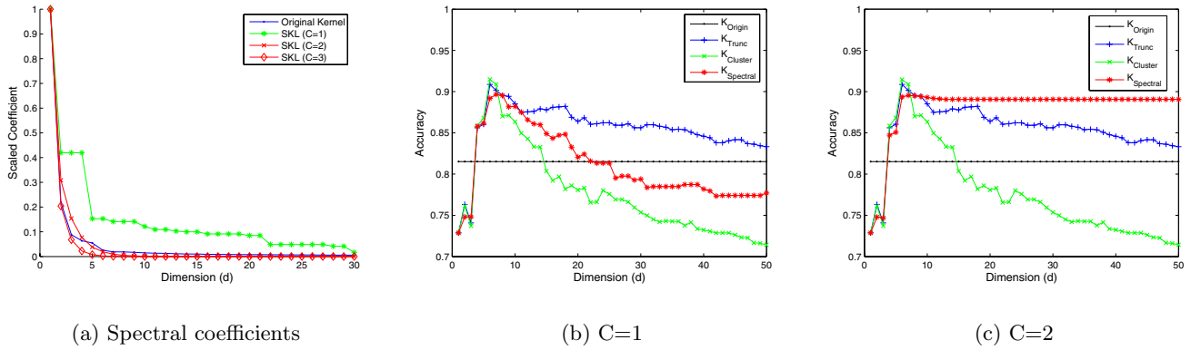
Figure 4: Example of Spectral coefficients and performance impacted by different decay factors on the Ionosphere dataset. The initial kernel is an RBF kernel and the number of labeled data is 20.
