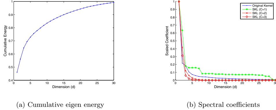
Figure 2: Illustration of cumulative eigen energy and the spectral coefficients of different decay factors on the Ionosphere dataset. The initial kernel is a linear kernel and the number of labeled data is 20.
